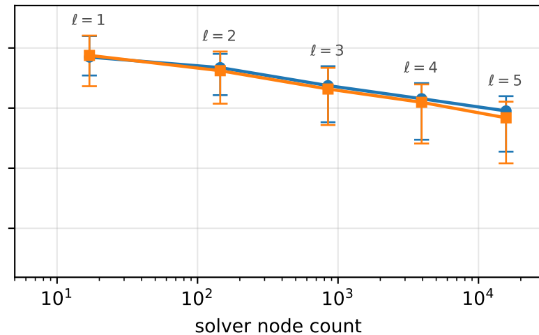
eight-dimensional model
