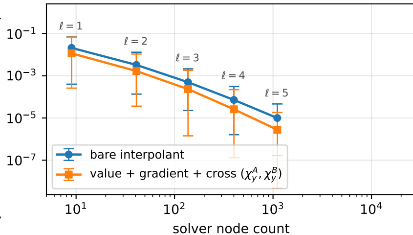
four-dimensional model
