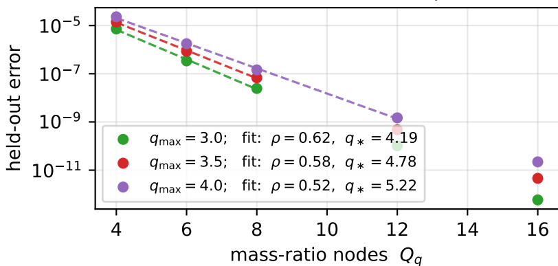
Mass-ratio wall — soft, complex
