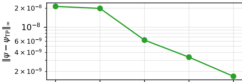
Quasi-circular field vs TP
