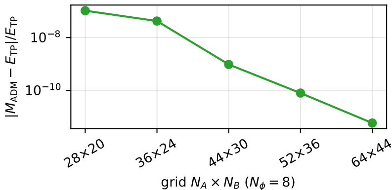
Quasi-circular ADM mass vs TP
