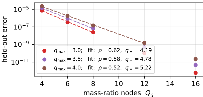
Mass-ratio wall — soft, complex
