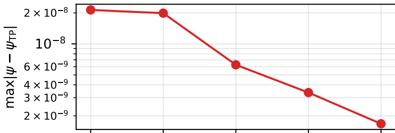
(a) quasi-circular field vs TP
