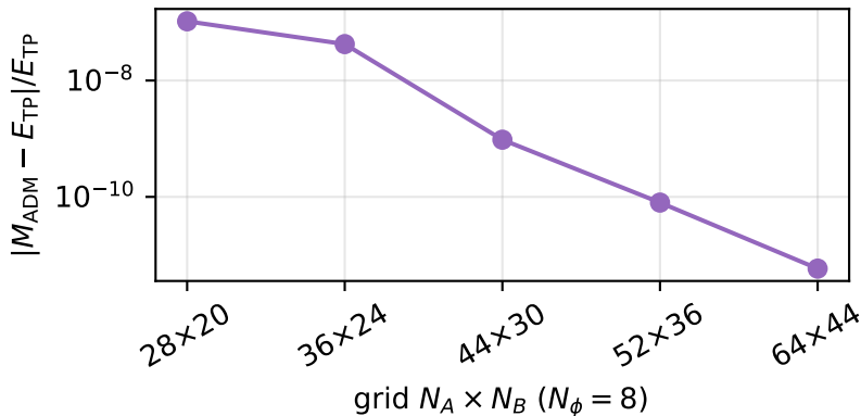
(b) quasi-circular ADM mass vs TP
