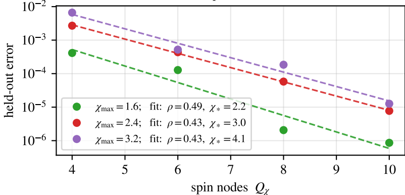
Spin wall
