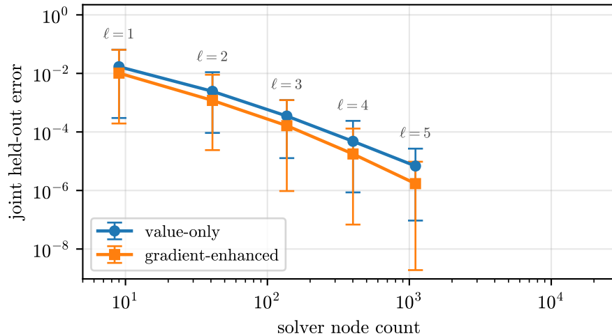
4D quasi-circular model: \theta = (b, q, \chi_y^A, \chi_y^B)
