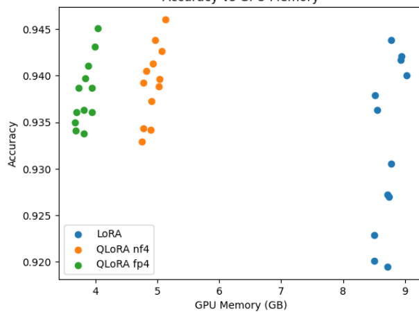
Accuracy vs GPU Memory
