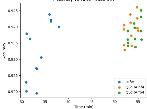
Accuracy vs Time (Trade-off)
