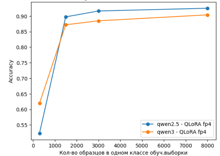
Accuracy vs Dataset Size for QLoRA (RU)
