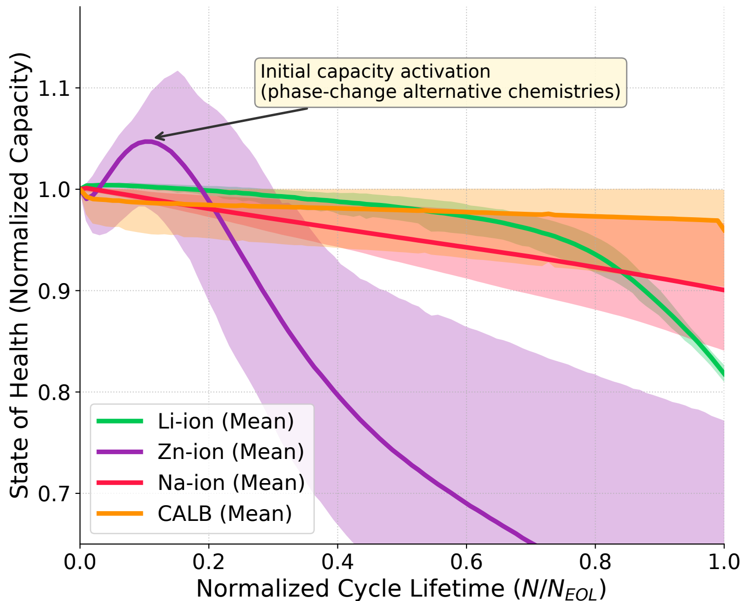
(a) Multi-Chemistry SOH Degradation Envelopes
