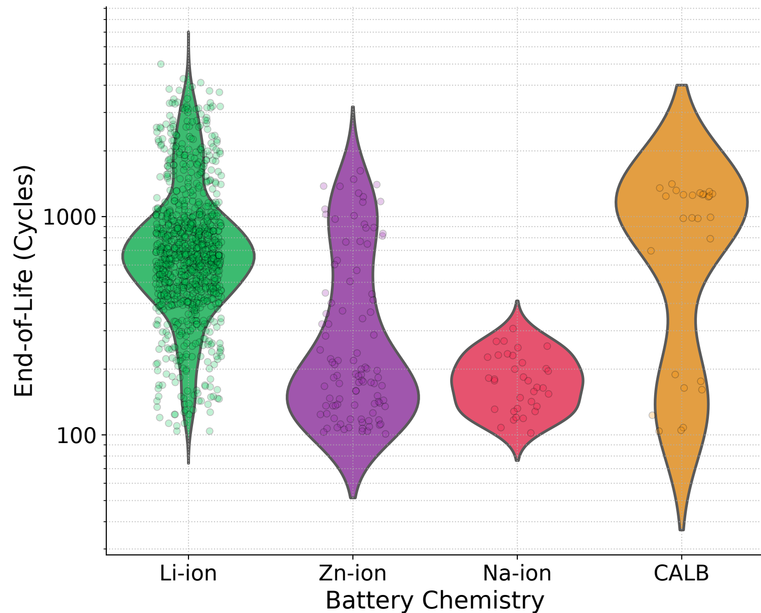
(b) Target EOL Cycle Life Distributions
