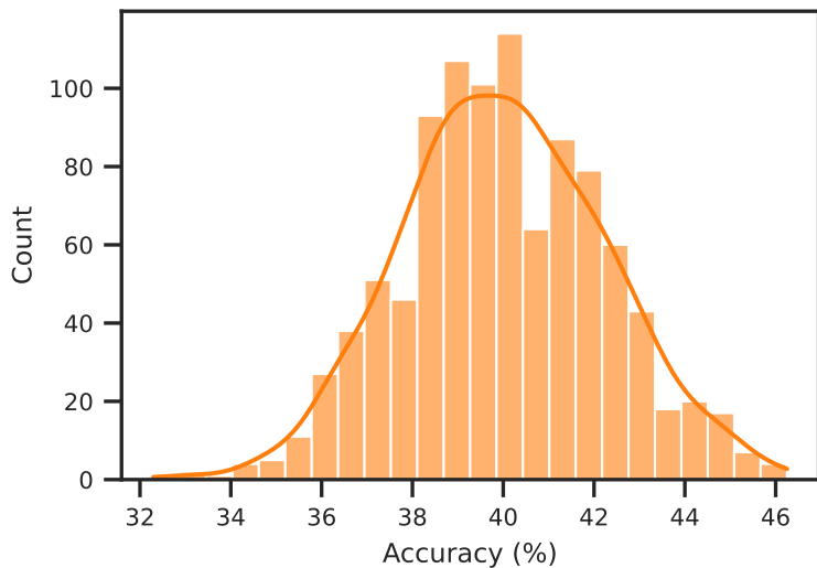
Na-ion Bootstrap Acc@15% (Mean: 40.0%)
