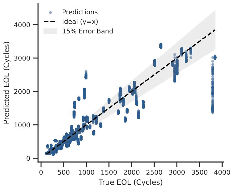
Na-ion Target vs Predicted EOL
