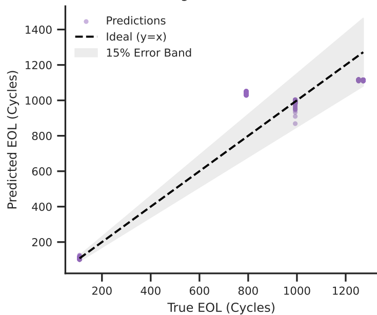
CALB Target vs Predicted EOL
