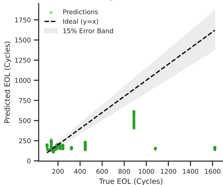
CALB Target vs Predicted EOL
