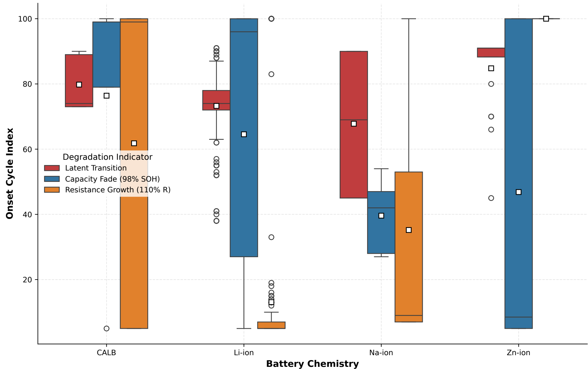
Comparison of Onset Detection Cycles Across Battery Chemistries
