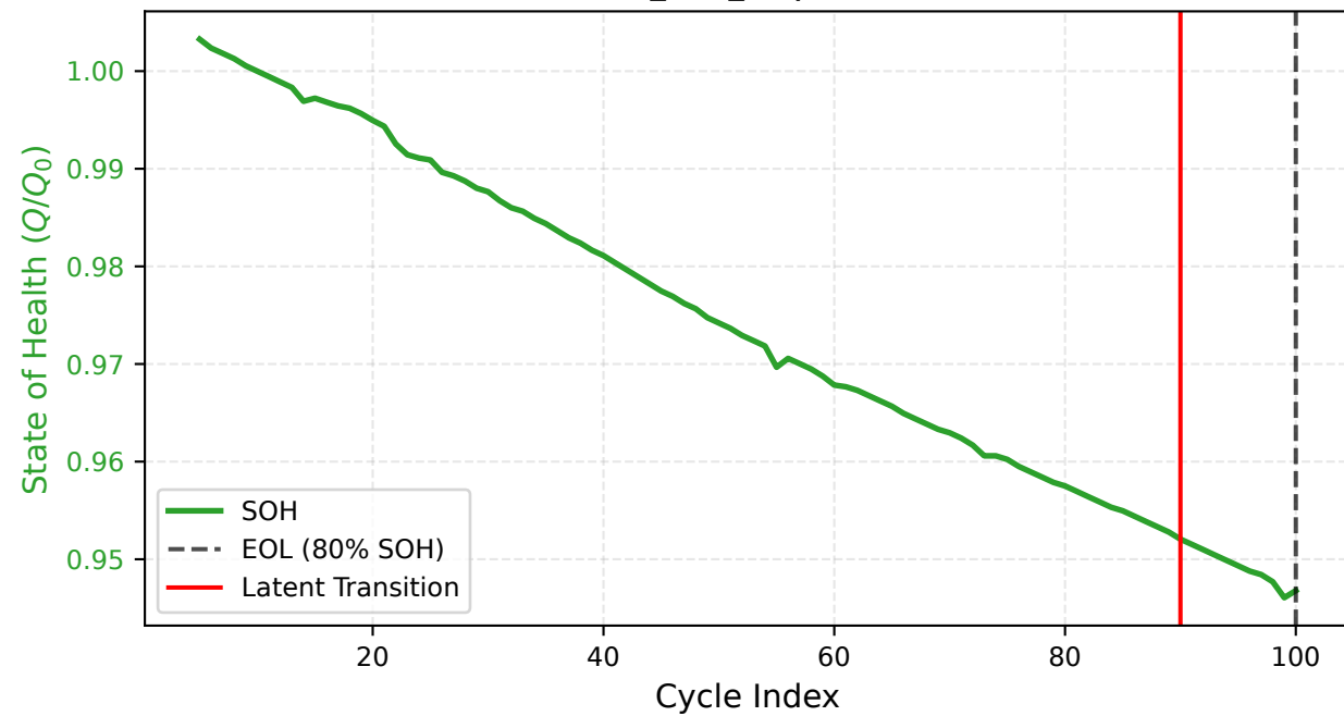
CALB (Cell: CALB_cell_3) | Conventional Metrics
