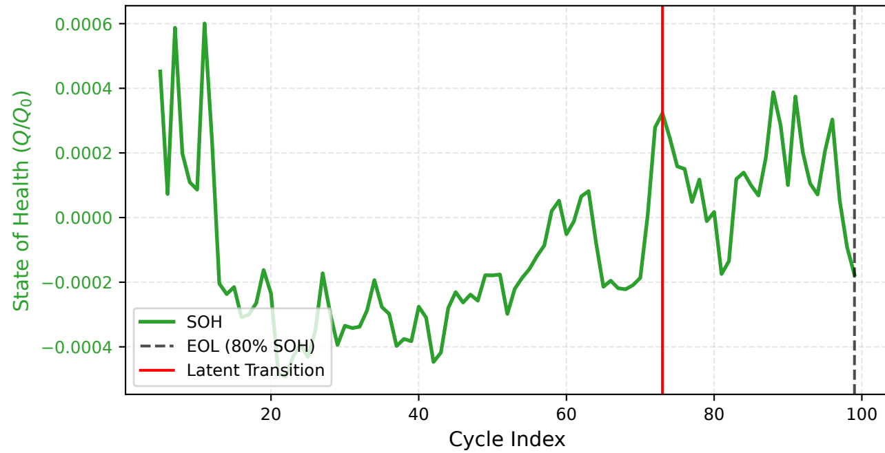
CALB (Cell: CALB_cell_3) | Conventional Metrics
