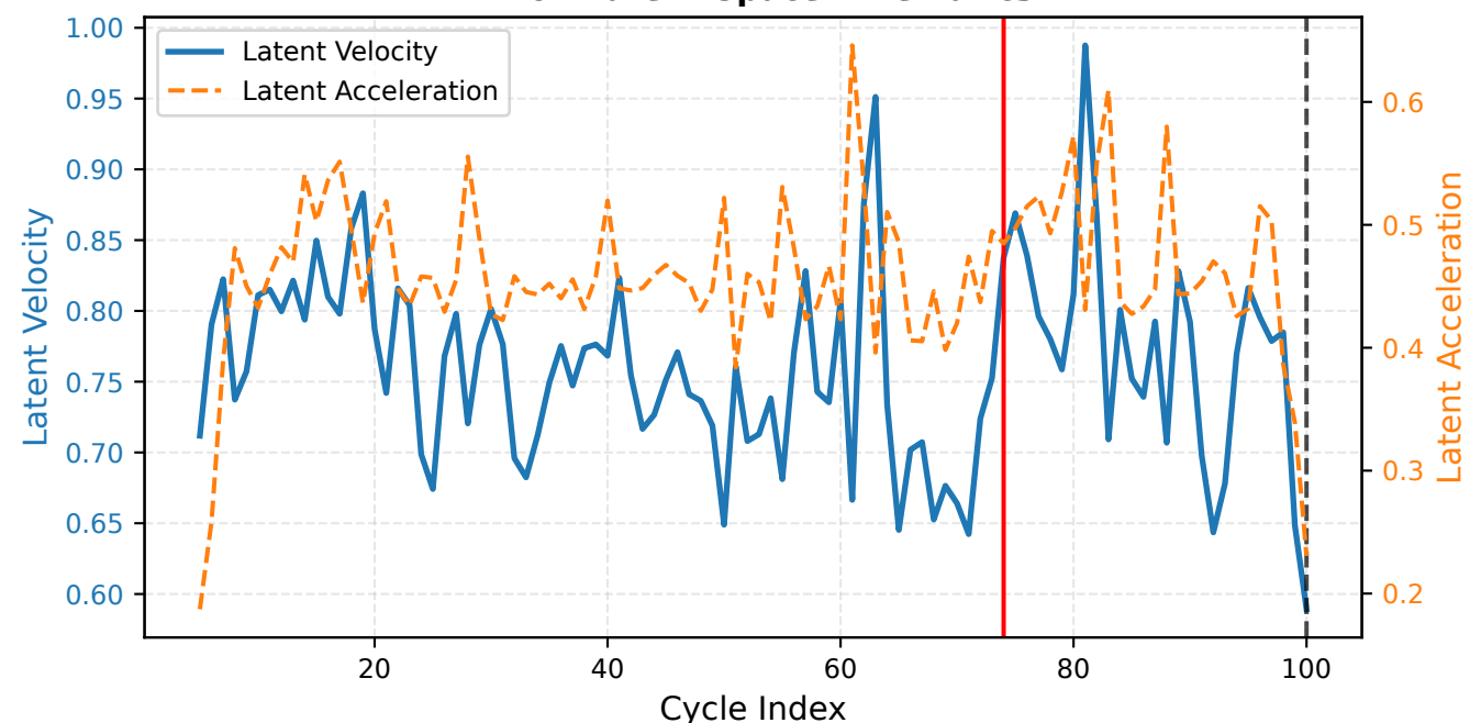
Zn-ion Latent Space Kinematics
