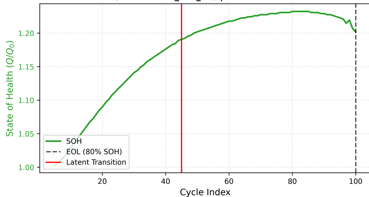
Na-ion (Cell: Na-ion_cell_2) | Conventional Metrics
