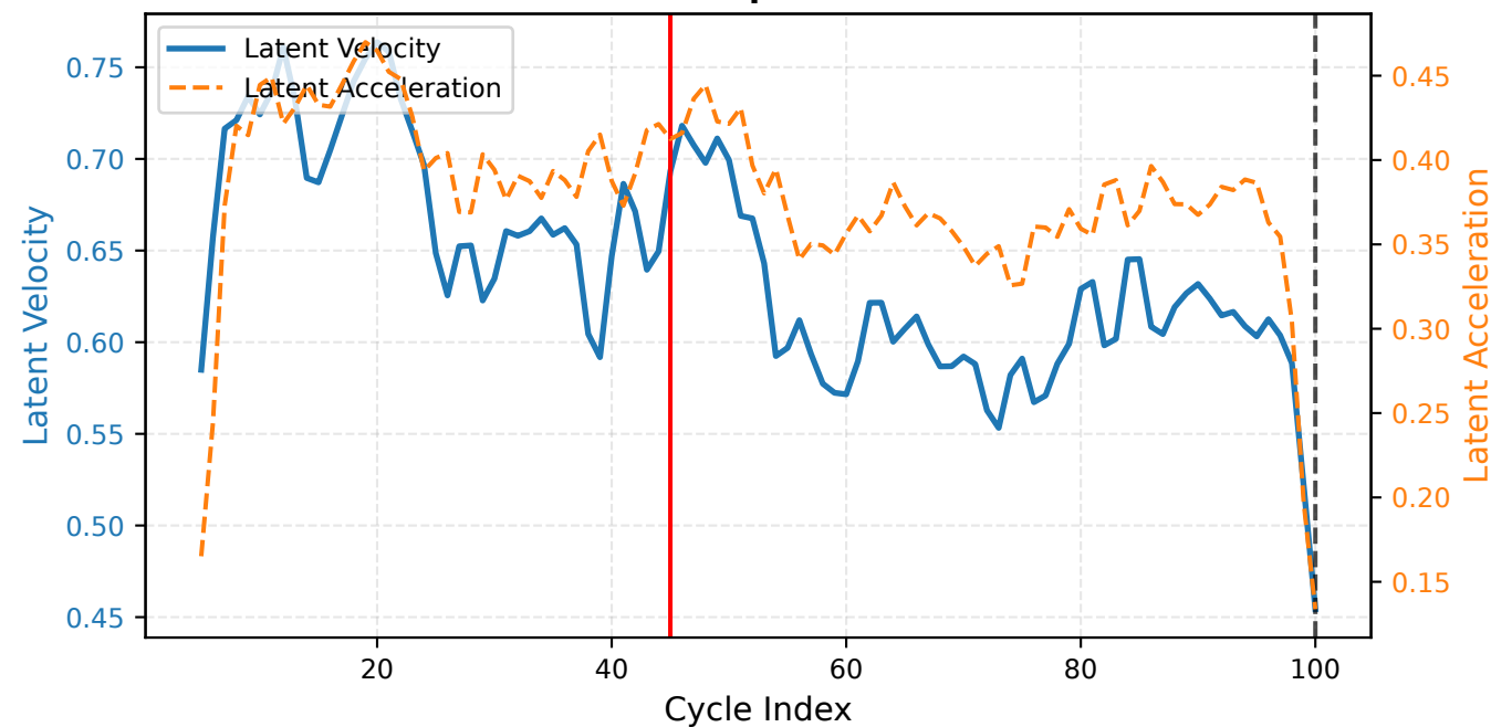
Na-ion Latent Space Kinematics
