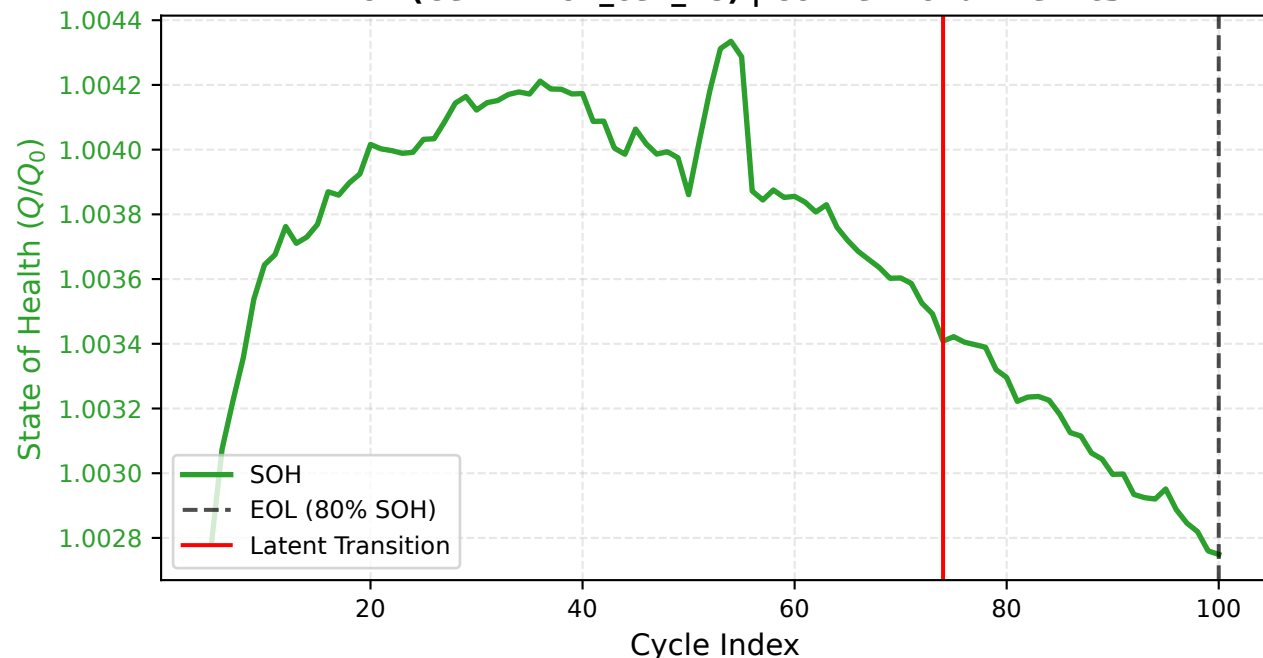
Zn-ion (Cell: Zn-ion_cell_18) | Conventional Metrics
