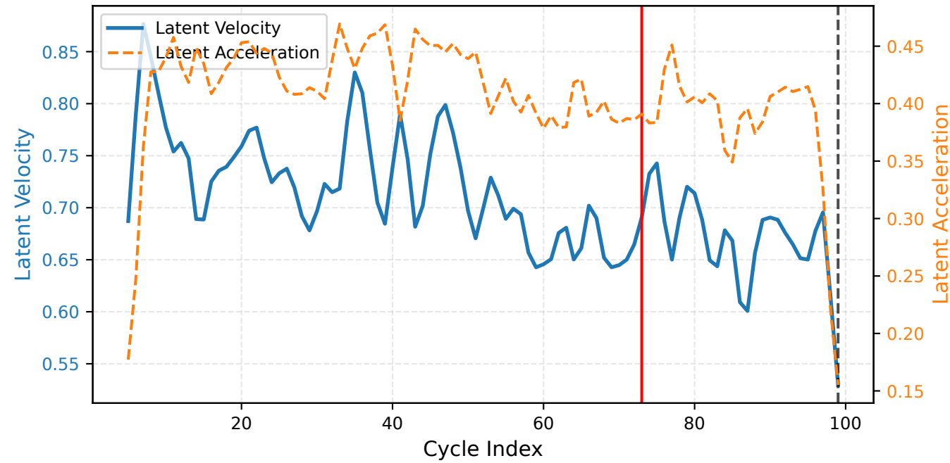
CALB Latent Space Kinematics
