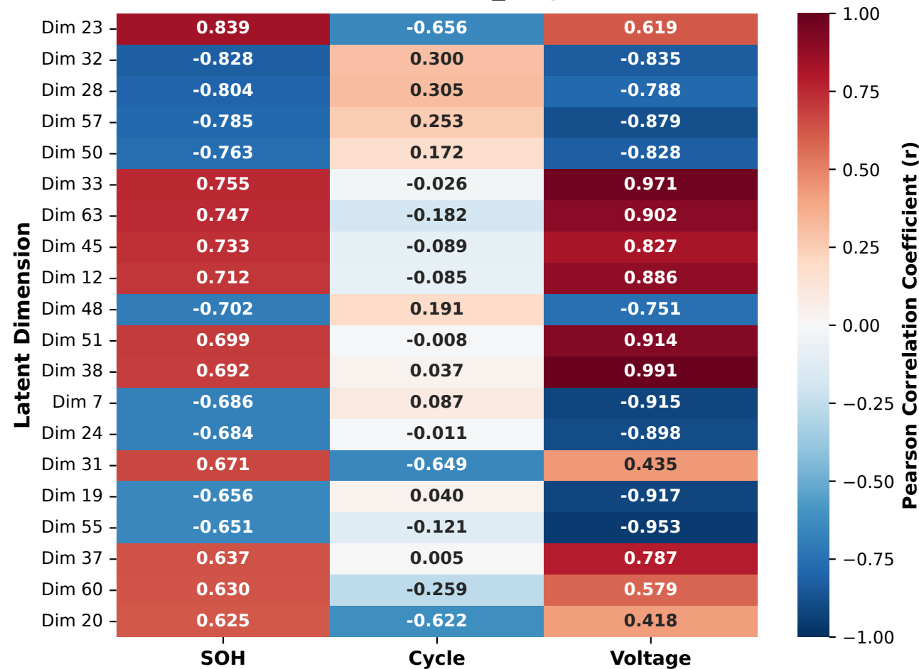
(c) Na-ion (NAion)
