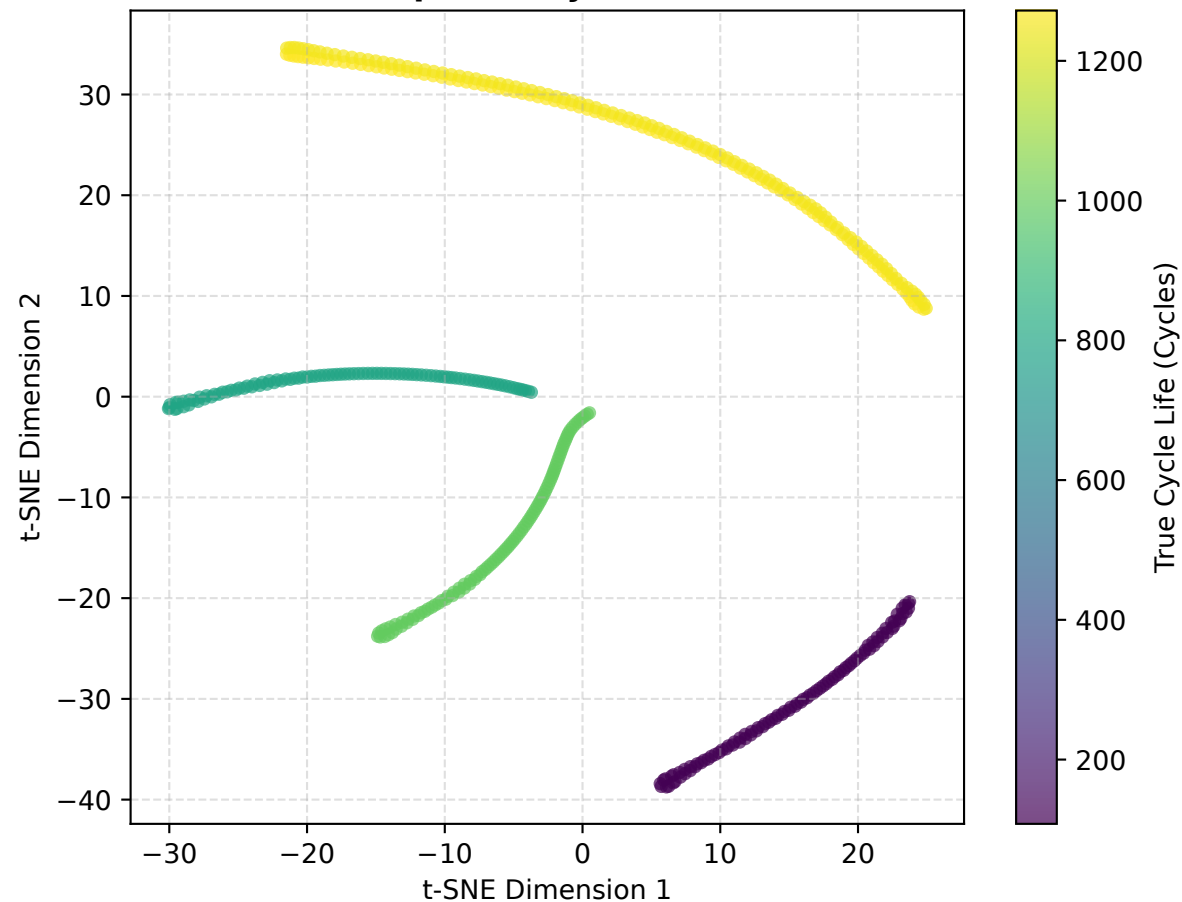
t-SNE Latent Space Projection: CALB (CALB)
