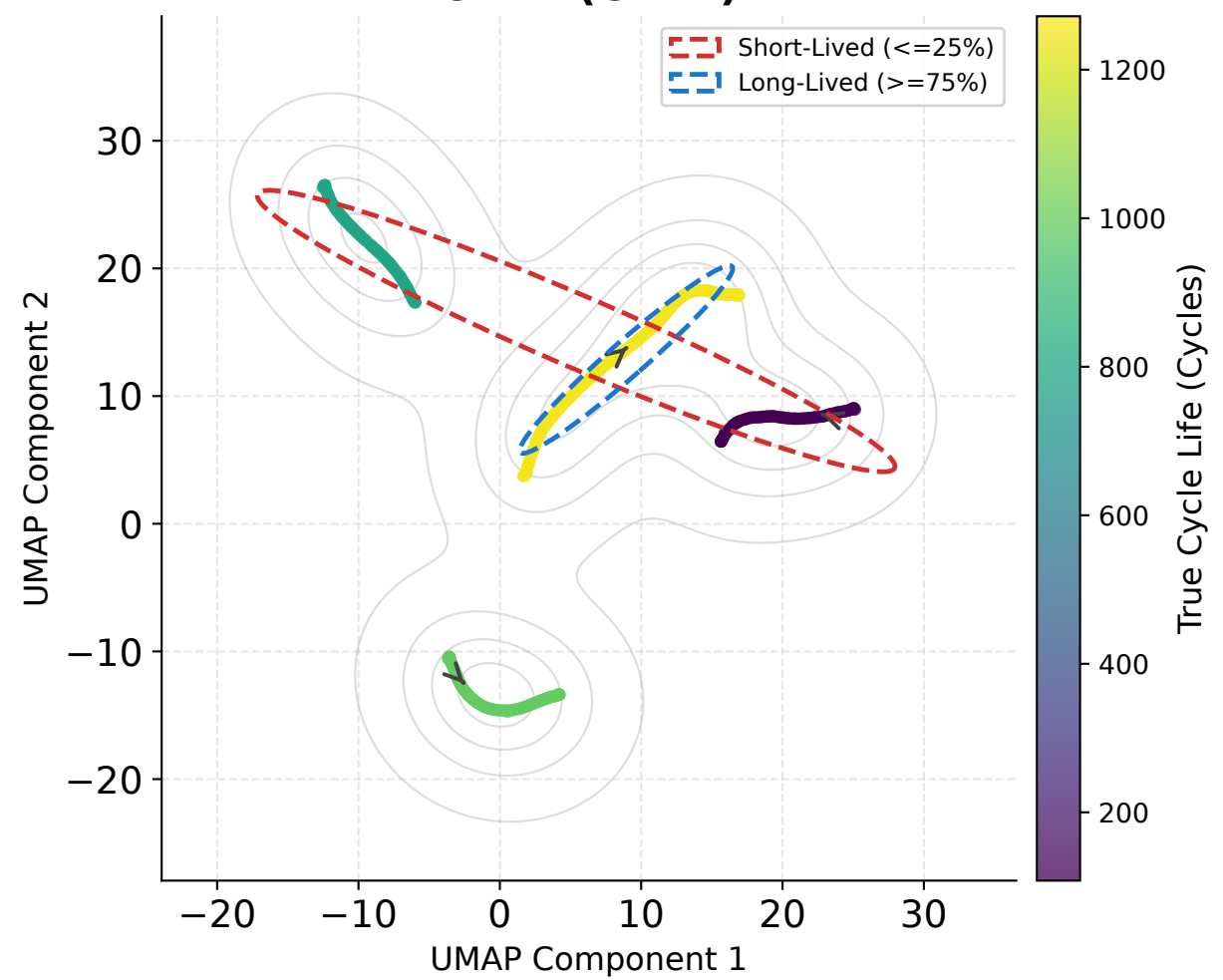
CALB (CALB)
