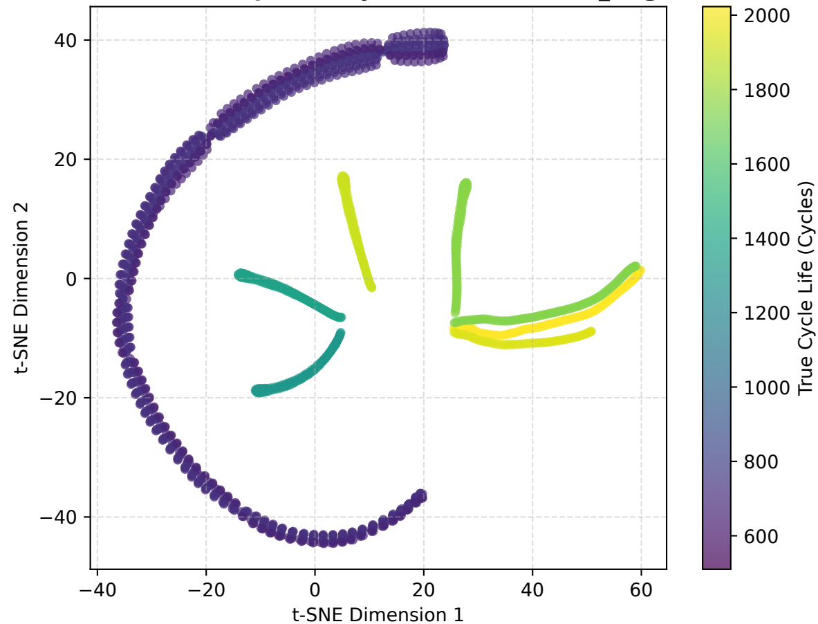
t-SNE Latent Space Projection: Li-ion (MIX_large)
