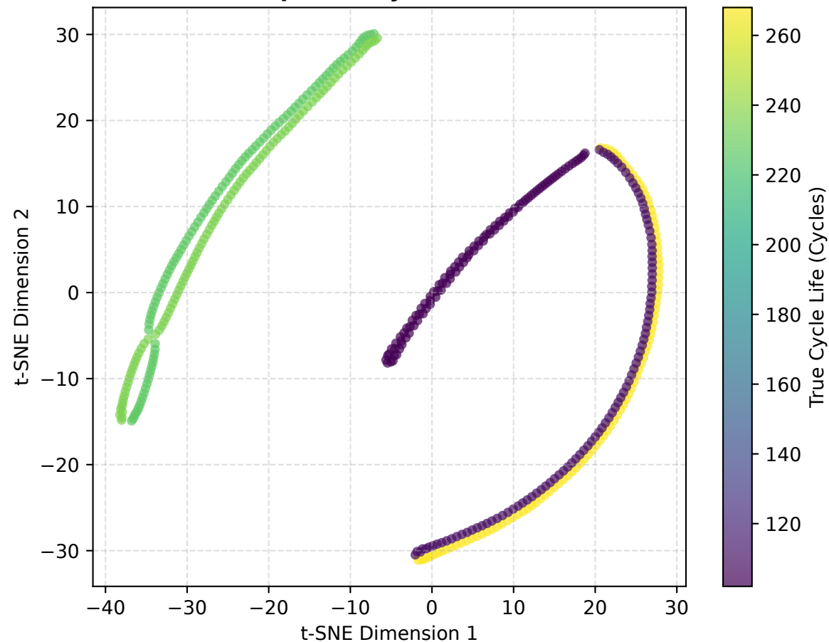
t-SNE Latent Space Projection: Na-ion (NAion)
