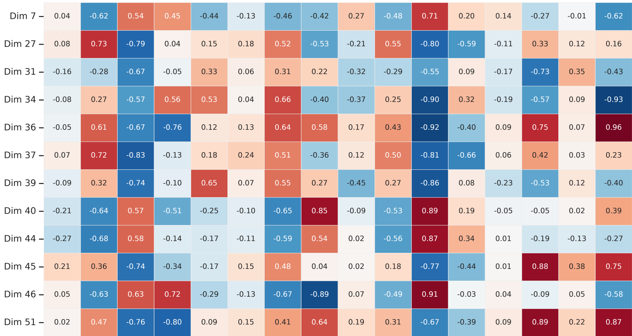
Universal Latent Dimensions Correlation Matrix across Batteries
