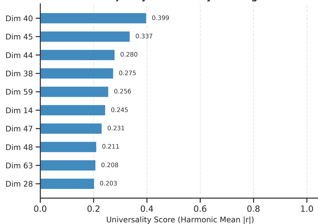
dQ/dV Peak Universality Ranking
