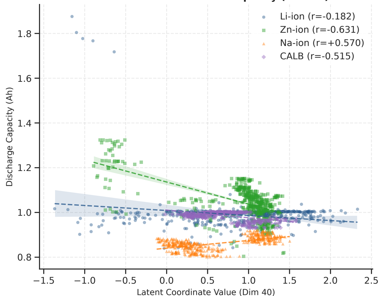
Universal Coordinates for Capacity (Dim 40)
