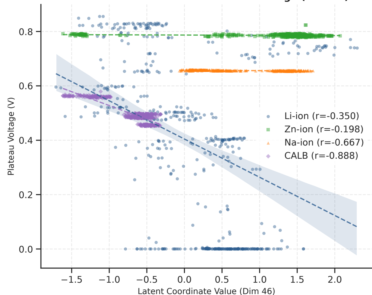
Universal Coordinates for Plateau Voltage (Dim 46)
