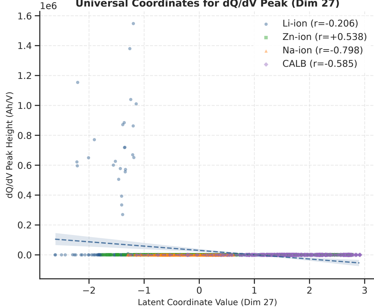
Universal Coordinates for dQ/dV Peak (Dim 27)
