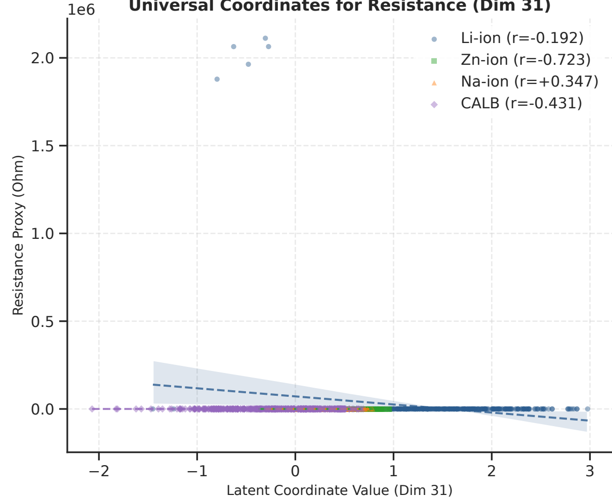
Universal Coordinates for Resistance (Dim 31)
