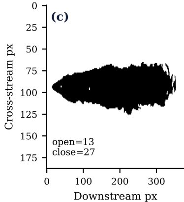
BW projection
