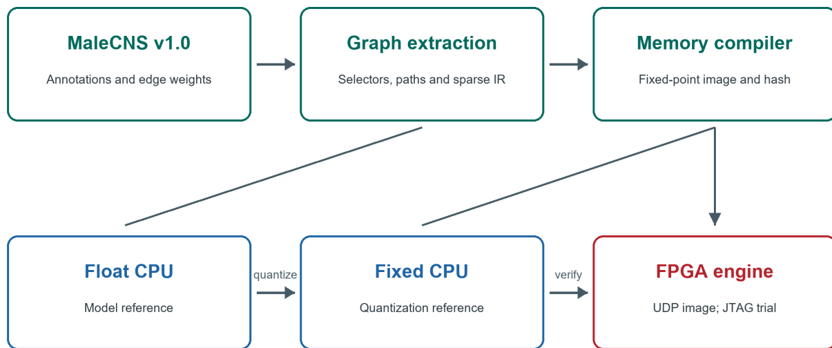
Figure 1. MaleCNS source tables feed path-constrained extraction and a fixed-point memory compiler. A runtime image may be loaded into the programmed FPGA over UDP; JTAG controls the recorded trials. The floating CPU, fixed CPU, RTL, and FPGA occupy distinct verification levels. Arrows describe data and comparison flow, not anatomical connectivity.
