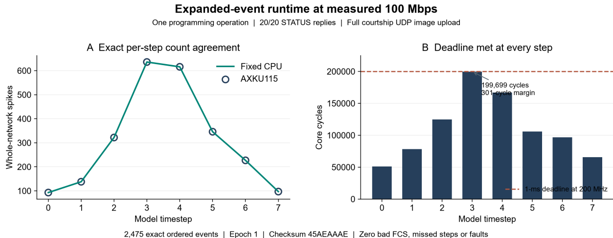
Figure 10. Additional speed-controlled trial on the same expanded-event bitstream at an actual 100-Mbps link. (A) Fixed-CPU and board whole-network spike counts coincide at all eight steps; a separate raw-event audit matched all 2,475 ordered events. (B) Core step cycles remain below the 200,000-cycle deadline, with a 301-cycle minimum margin. The recorded session also passed 20/20 STATUS probes and a complete courtship UDP image upload, with zero post-trial bad FCS. These results describe one eight-step session and do not establish 1-Gbps reliability or long-trial performance at 100 Mbps.
