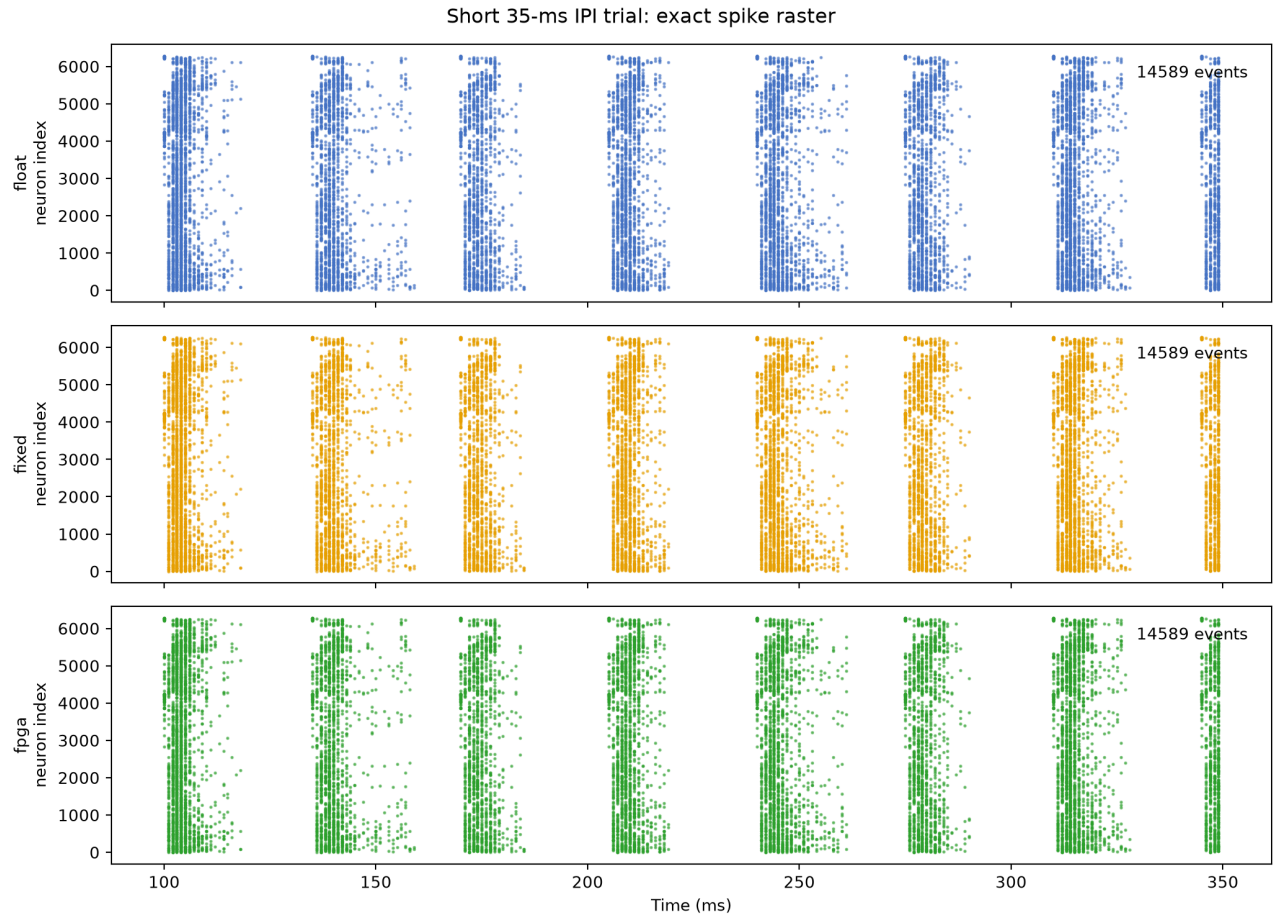
Figure 3. Full individual-event raster for the 350-ms, eight-pulse courtship trial. CPU float, CPU fixed, and FPGA output agree on the ordered event sequence. The original runtime P0 long trials were verified through per-step group counts because their event capture was disabled; a separate expanded-event bitstream later captured three complete long sequences (Figure 9).
