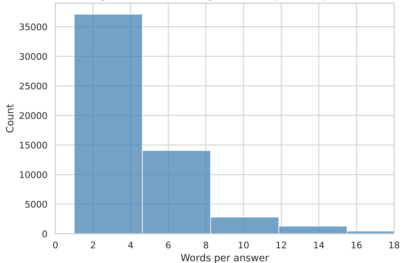
gemma — answer length in words (positive spans)
