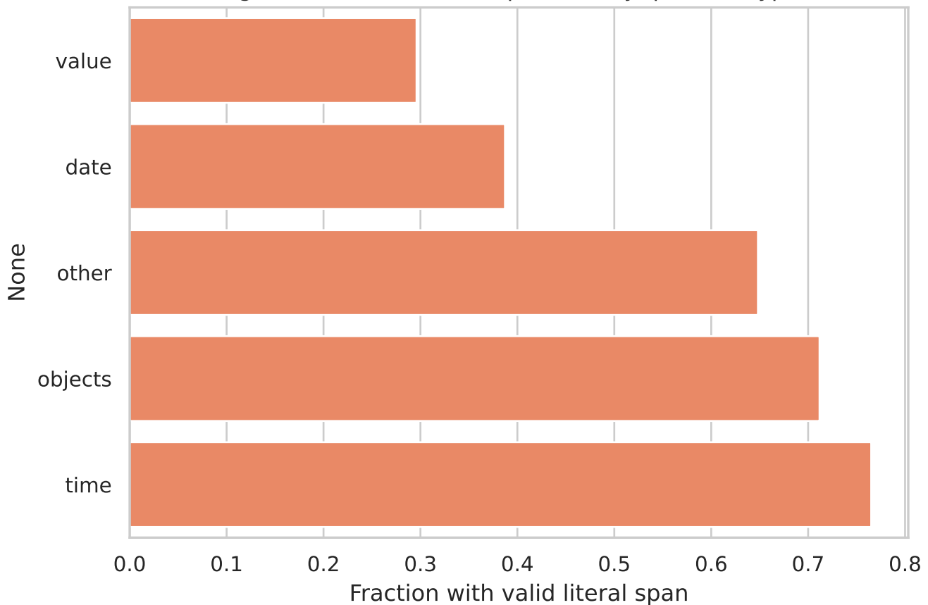
gemma — valid literal-span rate by question type
