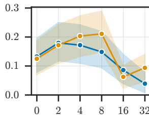
self-kill rate
