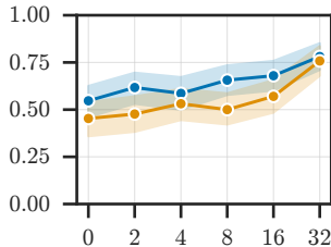
win rate
