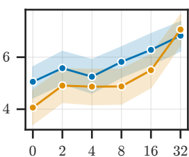
score
