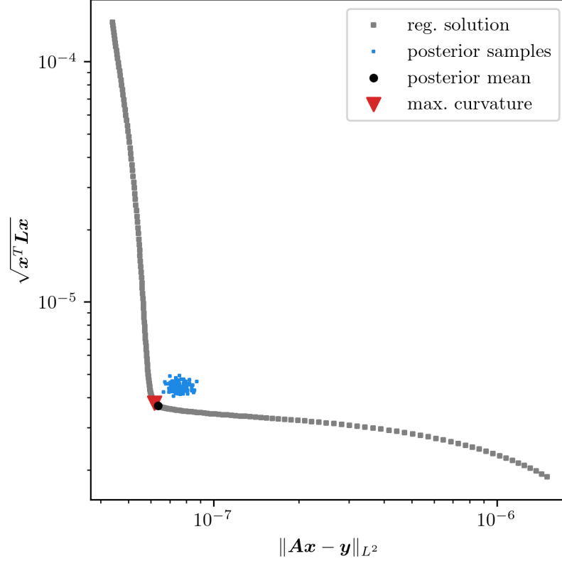
Figure 4.8: L-curve of regularisation norm \sqrt{\mathbf{x}^T \mathbf{L} \mathbf{x}} against the data misfit norm \|\mathbf{A}\mathbf{x} - \mathbf{y}\|_{L^2} for different \lambda values, where \mathbf{x}_\lambda is calculated as in Eq. 4.20. The regularised estimate is located at the point of maximum curvature (pink triangle) of the L-curve. Additionally, we calculate the data misfit norm and the regularisation norm for the mean (black circle) and samples (blue squares) of the full posterior of ozone.
