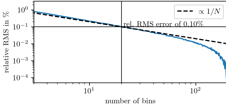
Figure 4.6: Relative RMS error of \boldsymbol{\mu}_{x|y} and covariance \boldsymbol{\Sigma}_{x|y} calculated by the weighted expectations and compared to a “ground truth” given by weighted expectations over 200 bins.
