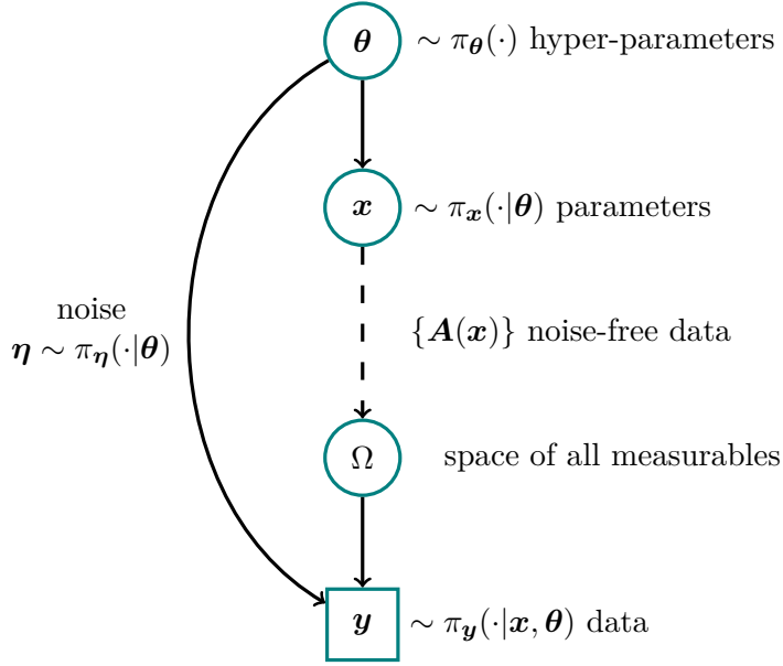
Figure 2.1: A directed acyclic graph (DAG) for an inverse problem visualises statistical dependencies as solid line arrows and deterministic dependencies as dotted arrows. The hyper-parameters \theta are distributed as (\sim) the hyper-prior distribution \pi(\theta) . The prior distribution \pi_x(\cdot|\theta) for the parameter x and the noise \eta \sim \pi_\eta(\cdot|\theta) are statistically dependent on some of those hyper-parameters. Then a parameter x \sim \pi_x(\cdot|\theta) is deterministically mapped onto the space of all measurables \Omega through the forward model A(x) . From the space of all measurable noise-free data we observe (square box) a data set y = A(x) + \eta with some additive random noise, which determines the likelihood function \pi(y|x, \theta) .
