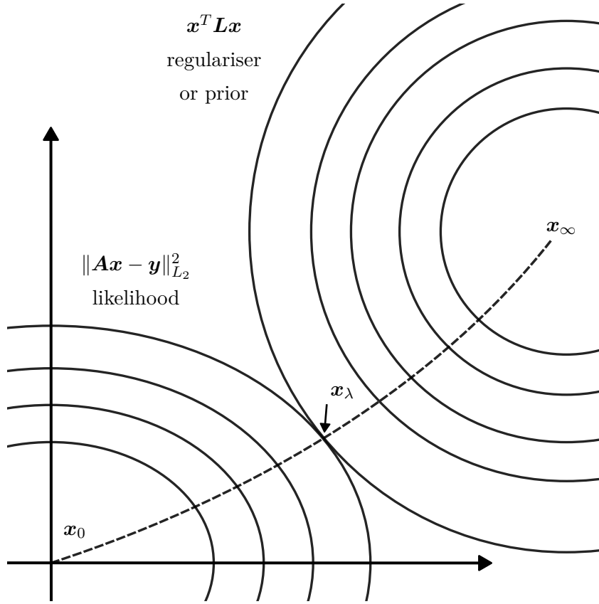
Figure 2.3: This Figure is not to scale and directly inspired by [20]. One regularisation solution \mathbf{x}_\lambda is obtained by following a contour line \|\mathbf{Ax} - \mathbf{y}\|_{L_2}^2 = c until \mathbf{x}^T \mathbf{Lx} is minimised. \lambda is the regularisation parameter or Lagrange multiplier and ranges from 0 to \infty . In the centre of the likelihood contours a solution \mathbf{x}_0 unaffected by the regulariser is obtained, whereas the solution \mathbf{x}_\infty is determined a-priori.
