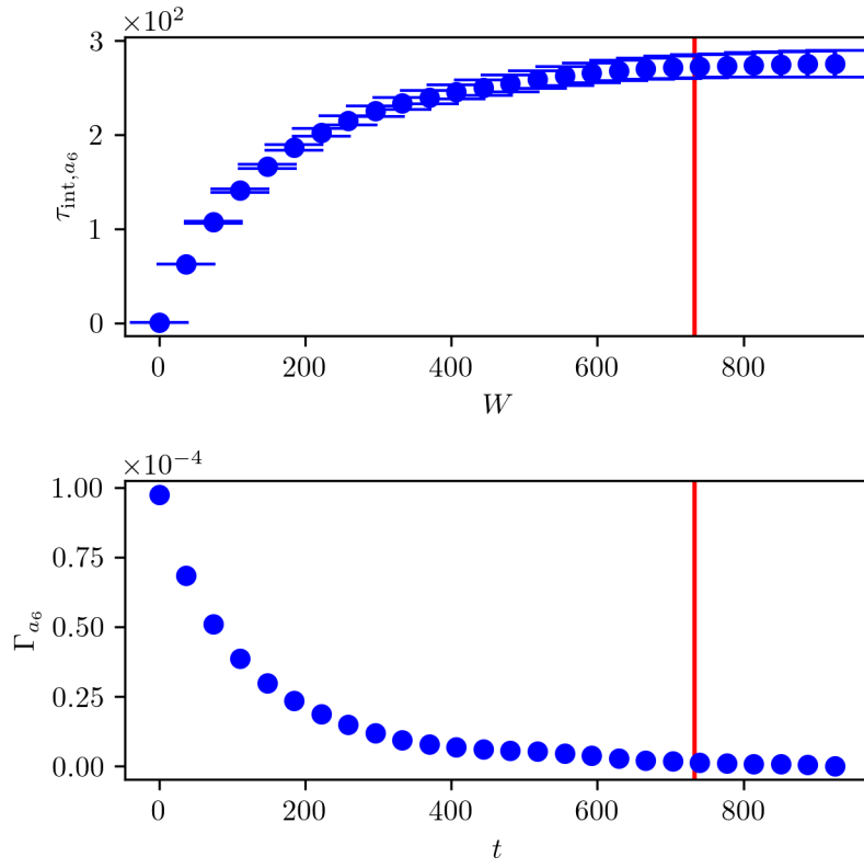
Figure B.26: The IACT \tau_{\text{int},a_6} at summation windows W and the estimated autocorrelation function \Gamma_{a_6} at lag t of samples a_6 \sim \pi(\cdot|\mathbf{y}) from the t-walk for the approximated forward model. The estimated IACTs are twice the values provided by [30, 72].
