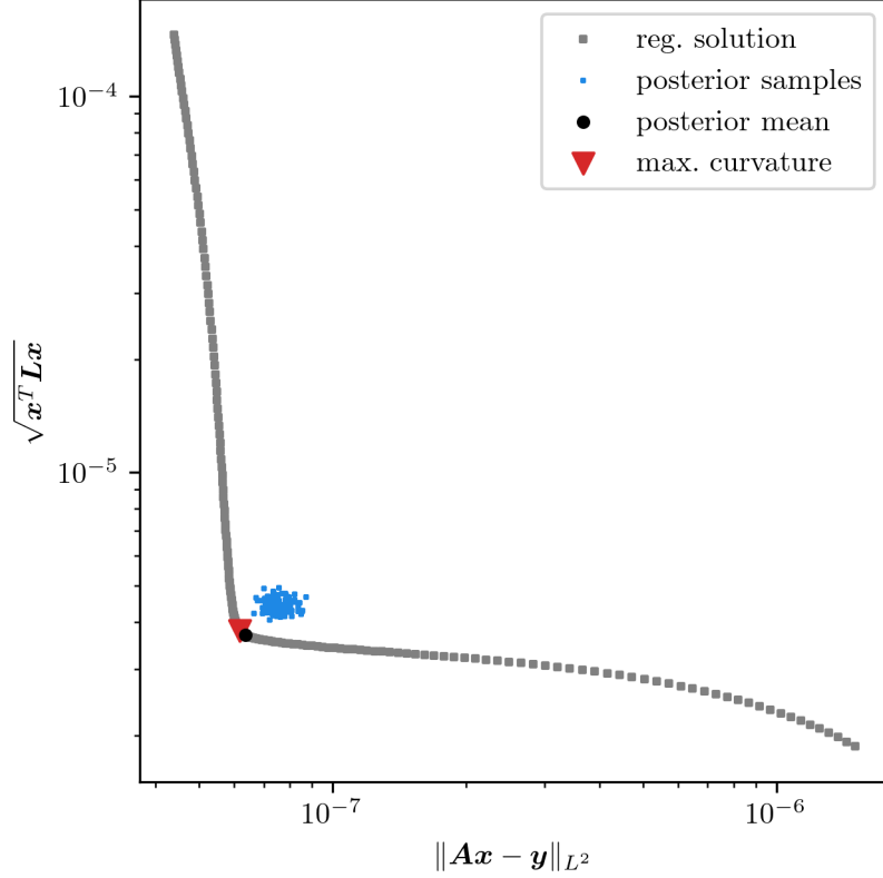
Figure 4.8: L-curve of regularisation norm \sqrt{x^T L x} against the data misfit norm \|Ax - y\|_{L^2} for different \lambda values, where x_\lambda is calculated as in Eq. 4.22. The regularised estimate is located at the point of maximum curvature (pink triangle) of the L-curve. Additionally, we calculate the data misfit norm and the regularisation norm for the mean (black circle) and samples (blue squares) of the full posterior of ozone.
