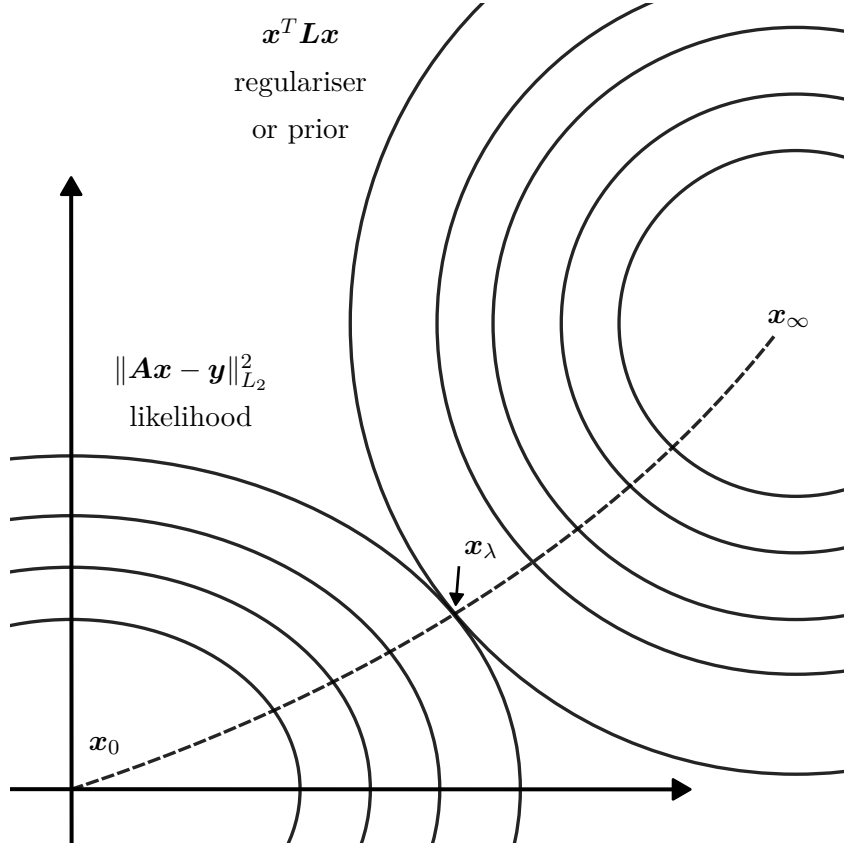
Figure 2.3: This Figure is not to scale and directly inspired by [21]. One regularisation solution \mathbf{x}_\lambda is obtained by following a contour line \|A\mathbf{x} - \mathbf{y}\|_{L_2}^2 = c until \mathbf{x}^T \mathbf{L} \mathbf{x} is minimised. \lambda is the regularisation parameter or Lagrange multiplier and ranges from 0 to \infty . In the centre of the likelihood contours a solution \mathbf{x}_0 unaffected by the regulariser is obtained, whereas the solution \mathbf{x}_\infty is determined a-priori.
