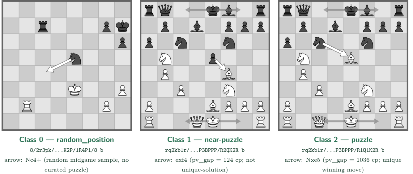
Figure 1: One representative example per class, rendered with crtk fen render . The class 1 and class 2 boards share the same CRTK sister parent ( crtk_parent_-1001373292417858425 ): the only structural difference is whether Bxe5 has been played. This makes the discriminator that distinguishes near-puzzle from puzzle as small as the data allows — a near-perfect ablation of the “unique-solution” property.
