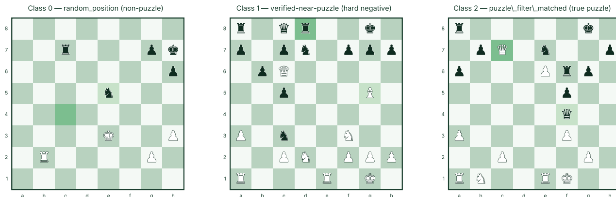
Figure 1: One representative example per class drawn from the train split. The from-square is shaded pale green, the to-square sage green. The hard-negative middle position ( fine_label 1 ) looks tactical but its pv_gap is only 27 cp — the architecture must learn to reject it. The right position ( fine_label 2 ) has a pv_gap of 838 cp and is a true puzzle.
