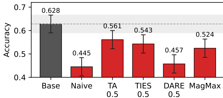
HumanEval pass@1
