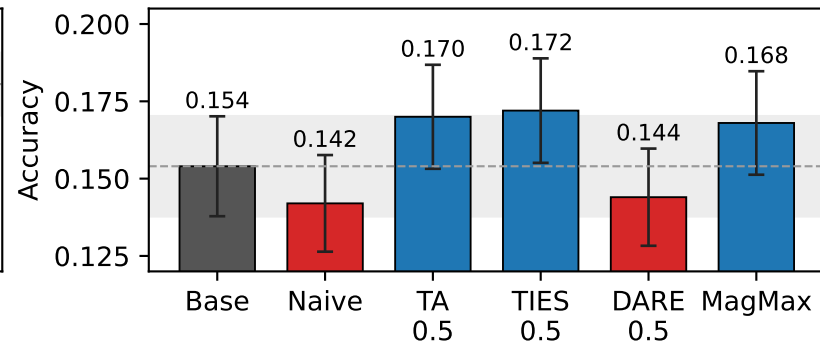
MATH-500 (4-shot)
