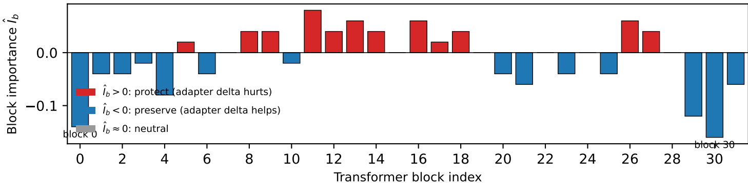
Per-block leakage-free importance \hat{l}_b on GSM8K (naive probe = 0.44)
