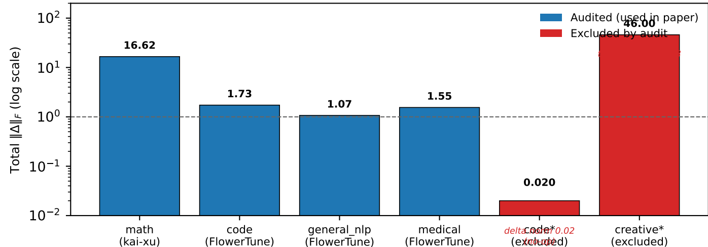
Adapter-audit outcome: 4 audited Llama-3.1 adapters + 2 excluded defective adapters
