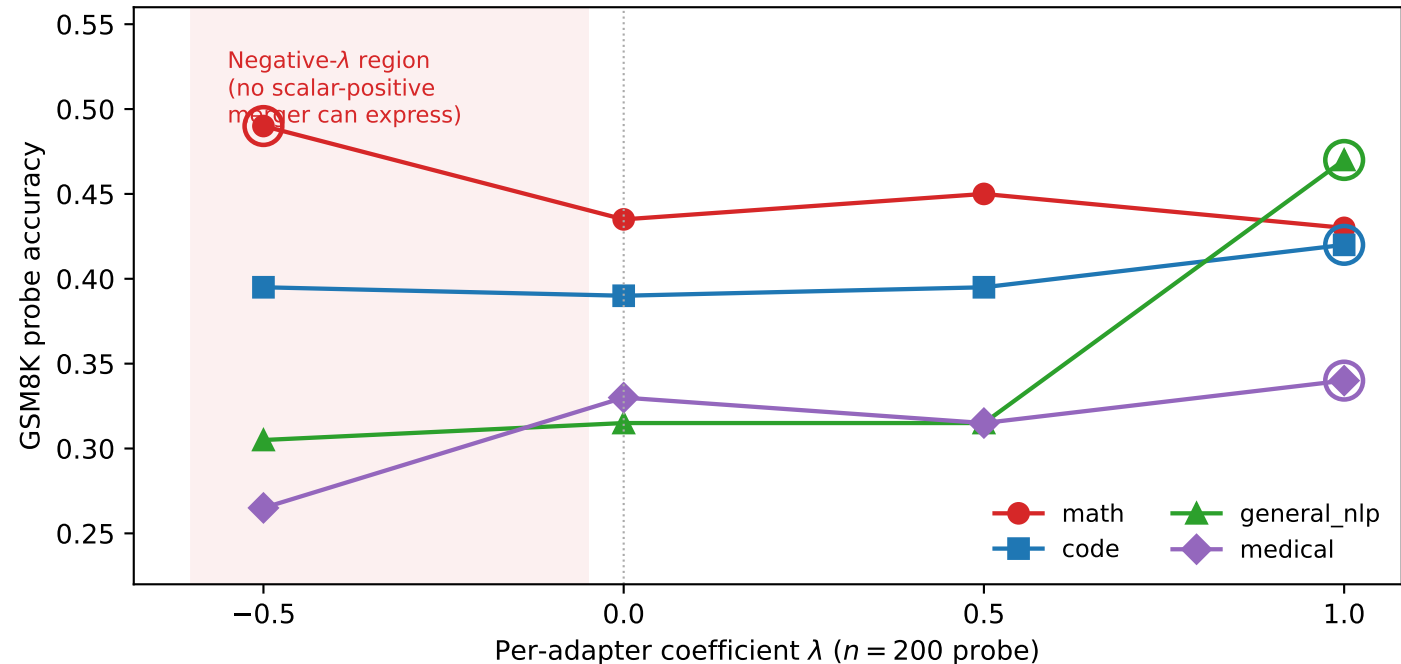
Probe accuracy vs. per-adapter \lambda . Math adapter is probe-optimal at \lambda = -0.5 .
