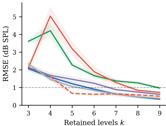
(a) Mean function comparison (active acquisition)
