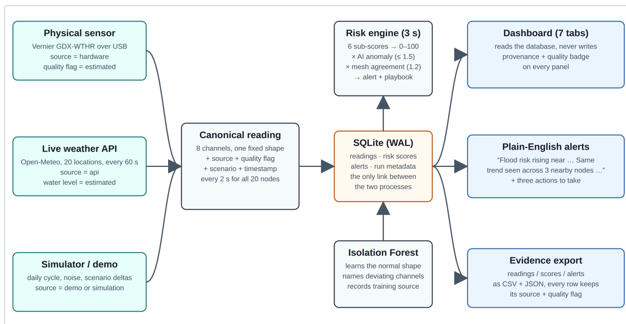
Figure 2 — The data path. Every source emits the same canonical reading (eight channels plus source and quality flag), so a real sensor is a drop-in and nothing downstream changes; one small database file is the only link between the engine and the dashboard.
