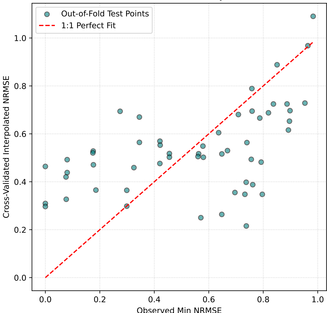
K-Fold Cross-Validation Accuracy ( R^2 = 0.246 )
