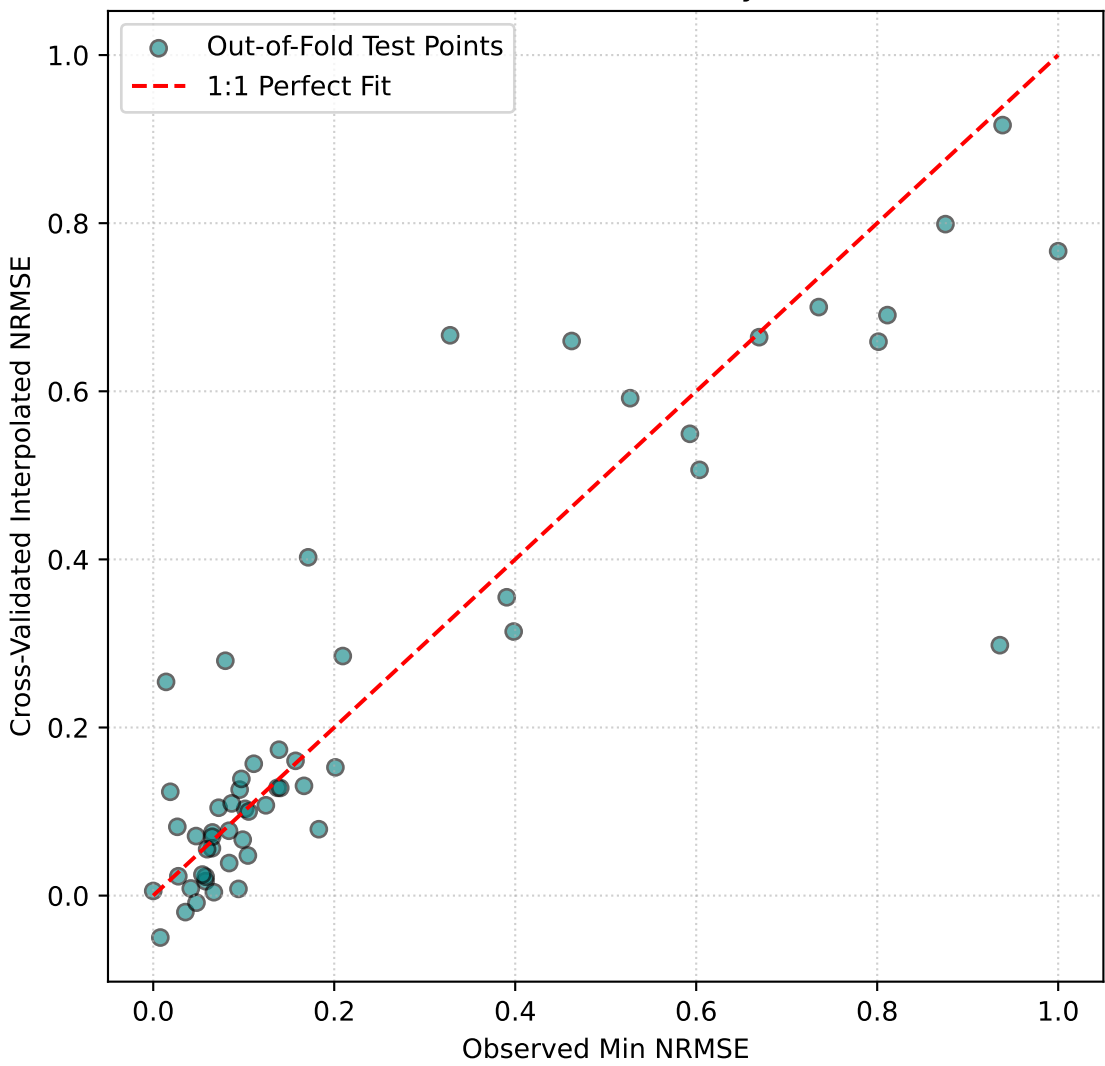
K-Fold Cross-Validation Accuracy ( R^2 = 0.800 )
