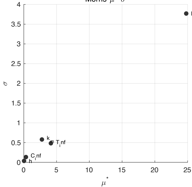
Morris \mu^* - \sigma
