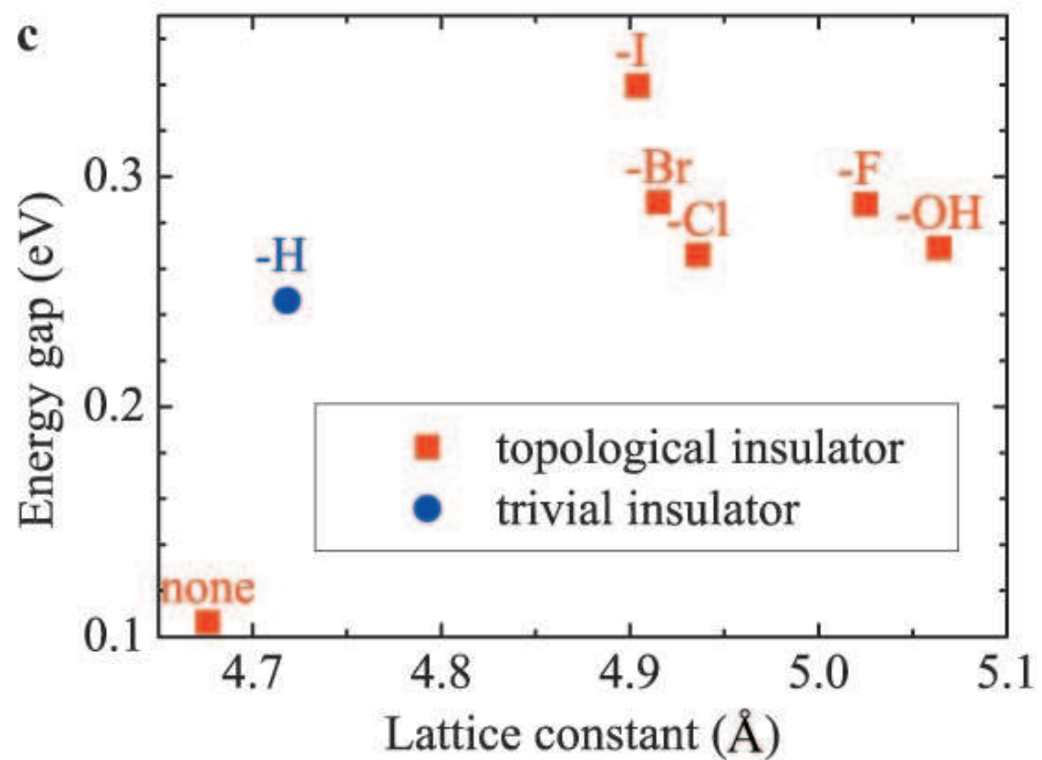
decorated stanene (2D SnX)
