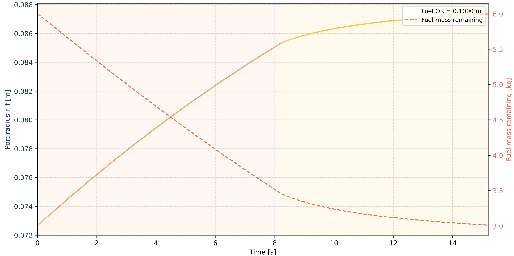
Fuel grain state vs. time (burn only)
