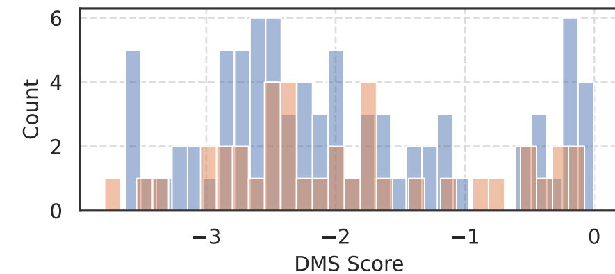
SQSTM MOUSE
