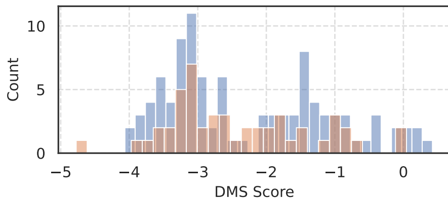
RD23A HUMAN
