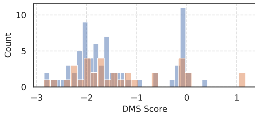
PIN1 HUMAN
