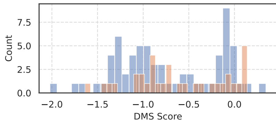
PIN1 HUMAN
