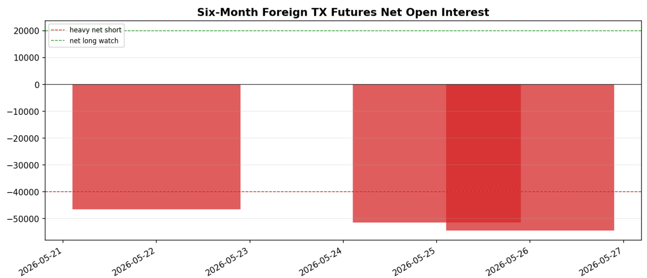
Chart 3: foreign_futures_net_oi_6m.png
