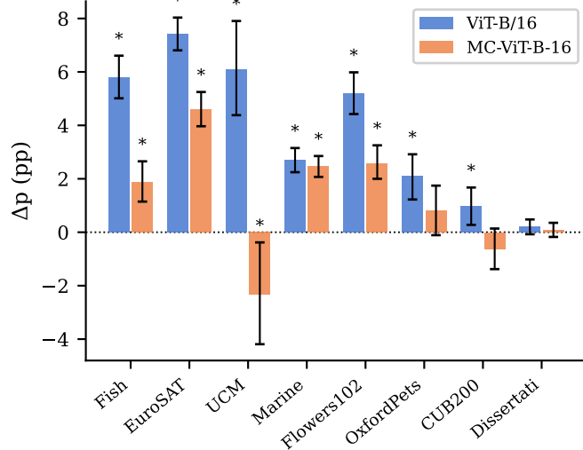
(b) Training data — same arch (ViT-B/16), different curation
