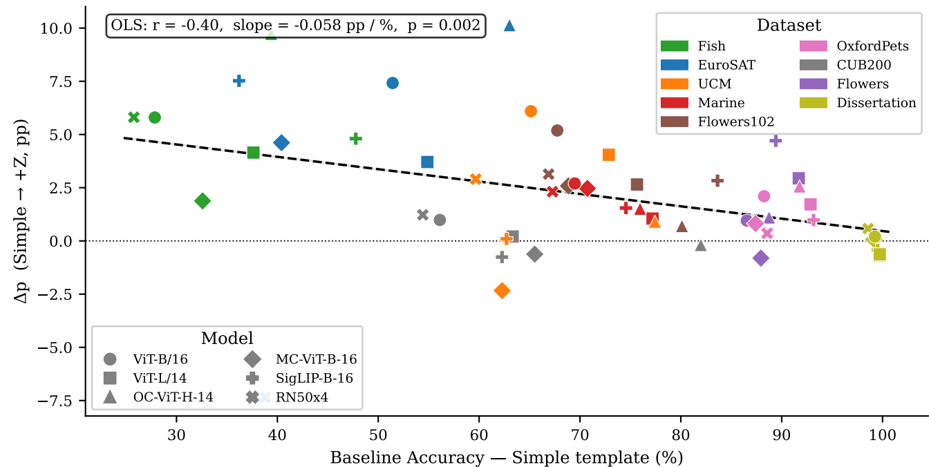
Contextual conditioning benefit vs. baseline accuracy
