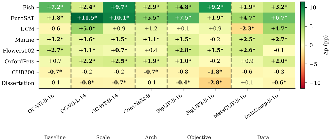
\Delta p across all datasets and model families (* = McNemar p < 0.05 )
