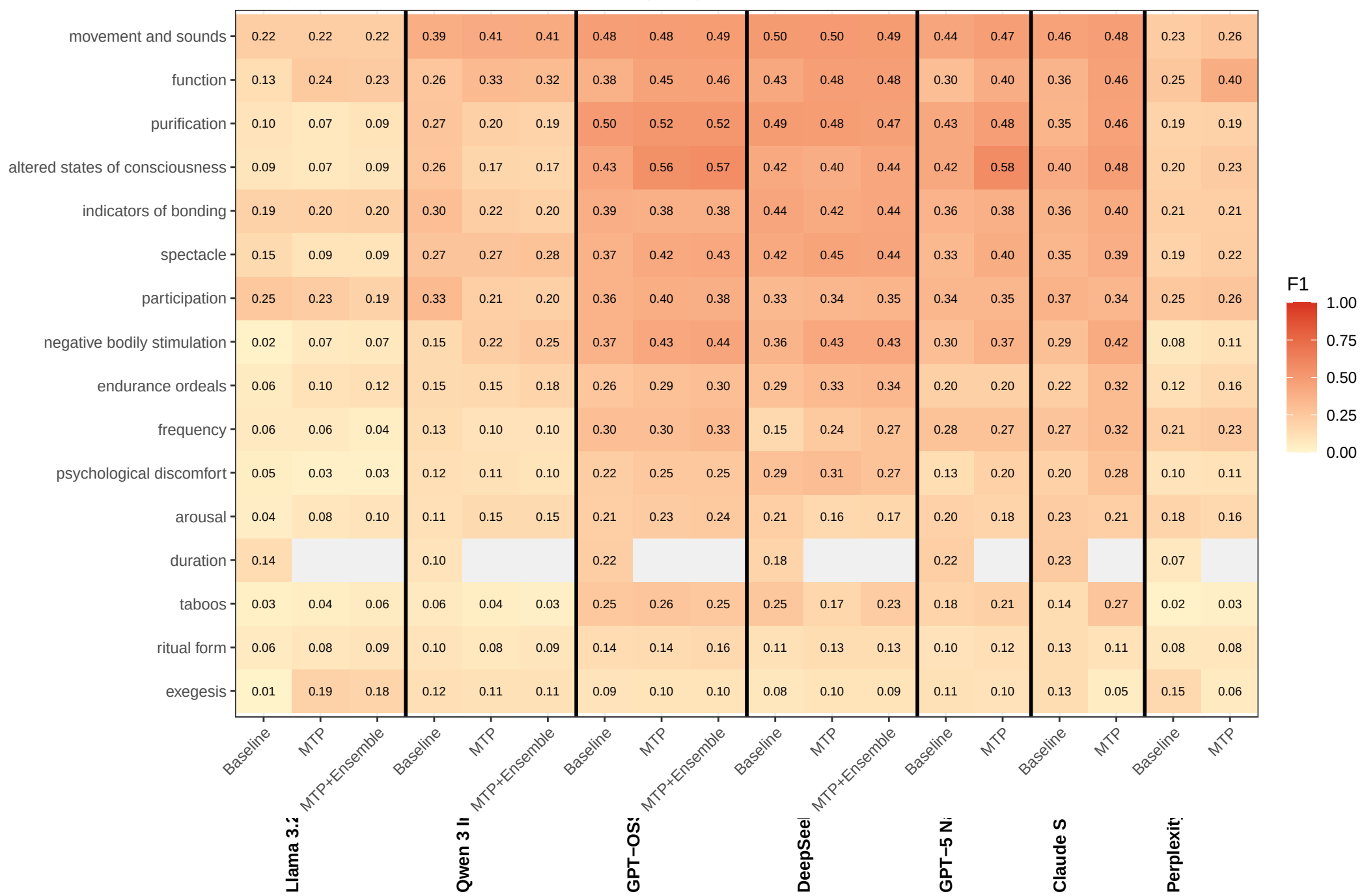
Category-level F1 Score by Model – Morphospace Features
