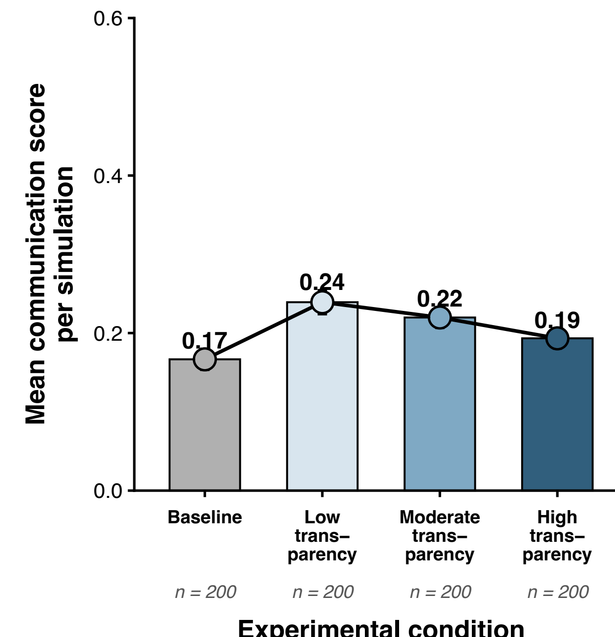
Figure 5: Mean communication quality scores (ranging from 0 to 1) across experimental conditions with 95% confidence intervals
