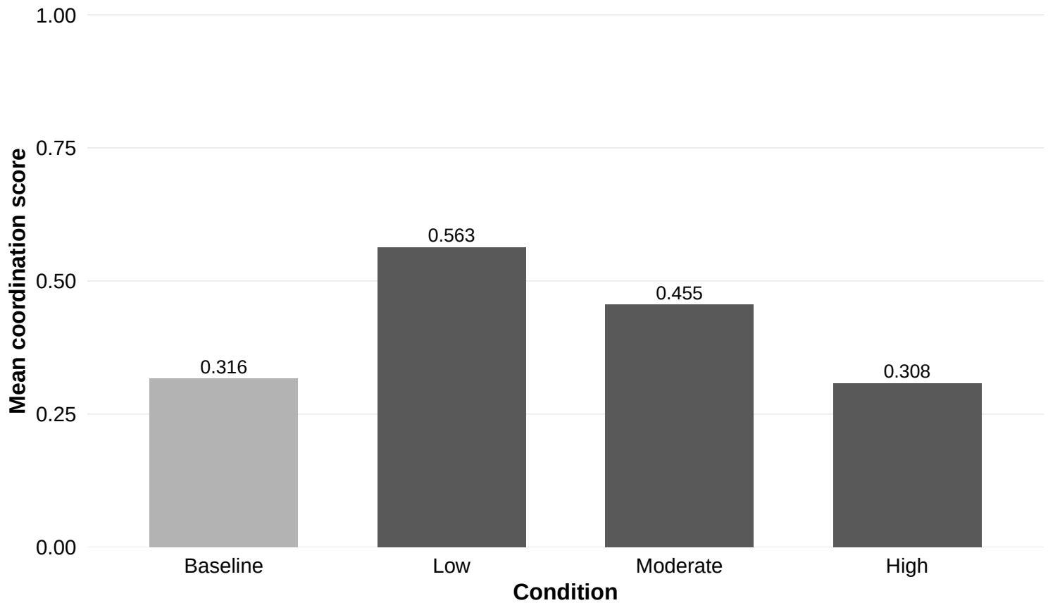
Mean team process coordination by condition
