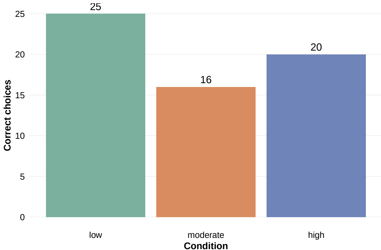
Correct candidate choices by condition (treatment)
